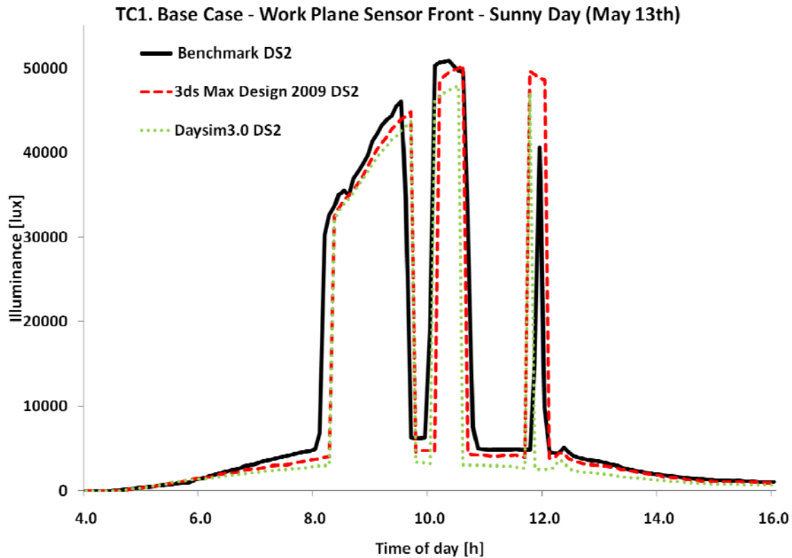
Figure 6: Measured and simulated illuminances for an upward facing work plane sensor close to the façade for TC1 (base case).
