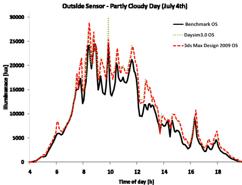
Figure 5: Measured and simulated vertical façade illuminances on the outside sensor on (a) a sunny and (b) a partly cloudy day.
