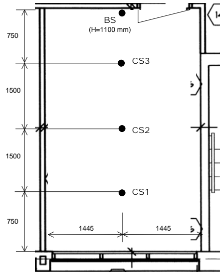
Figure 4: Inverted floor plan of the test space with the three ceiling illuminance sensors. Dimensions are in mm.
