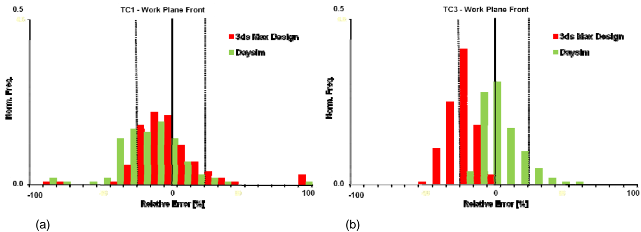
Figure 13: Frequency distribution of the relative error for the front work plane sensor for (a) TC1 (a) and (b) TC3.
