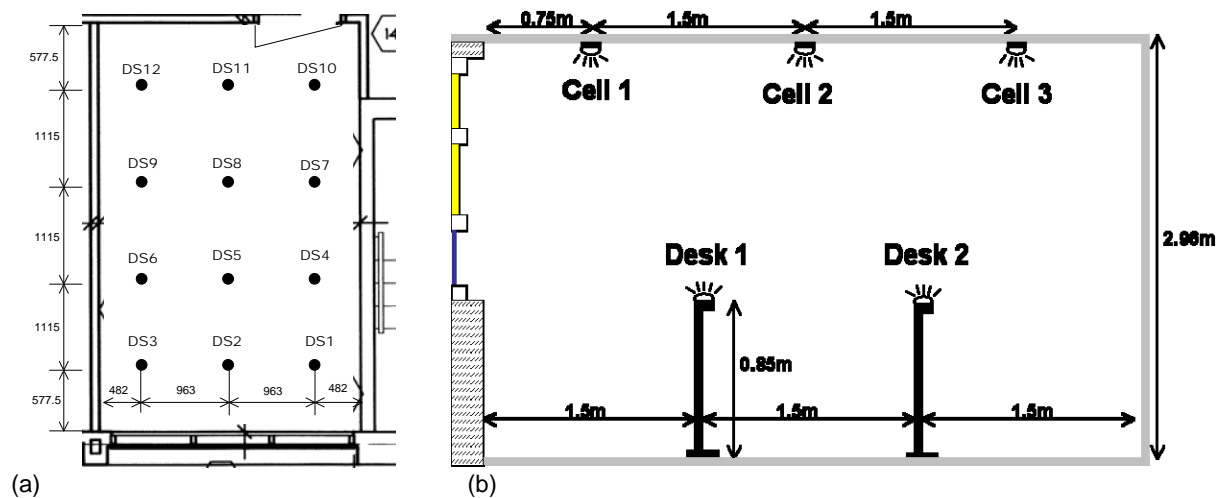
Figure 3: (a) Floor plan of the test space: For test cases TC1, TC2, TC4, and TC5 twelve work plane sensors were arranged in a three by four sensor grid, dimensions are in mm; (b) Section of the test space: For test case TC3 only two work plane sensors were collected.
