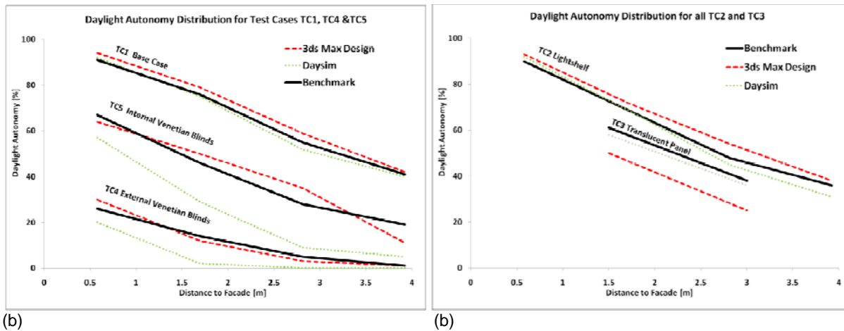
Figure 14: Daylight autonomies for the five test cases according to measurements and simulations.
