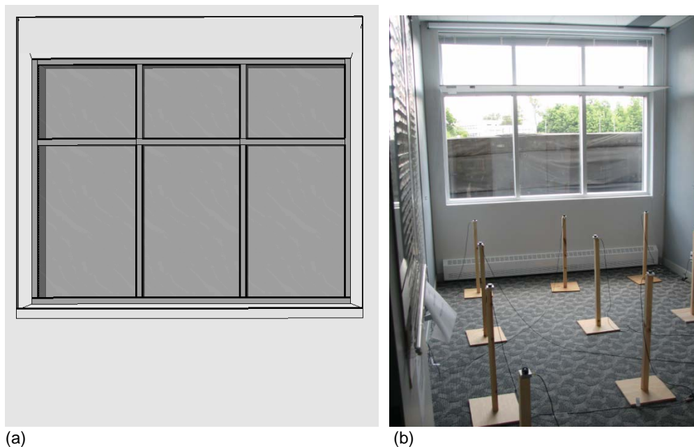
Figure 2: (a) Façade Section for TC1 Base Case; (b) internal view of the test room with the lightshelf.
