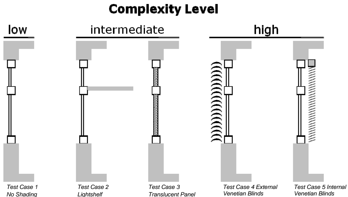
Figure 1: Façade sections of the five NRC daylighting test cases.
