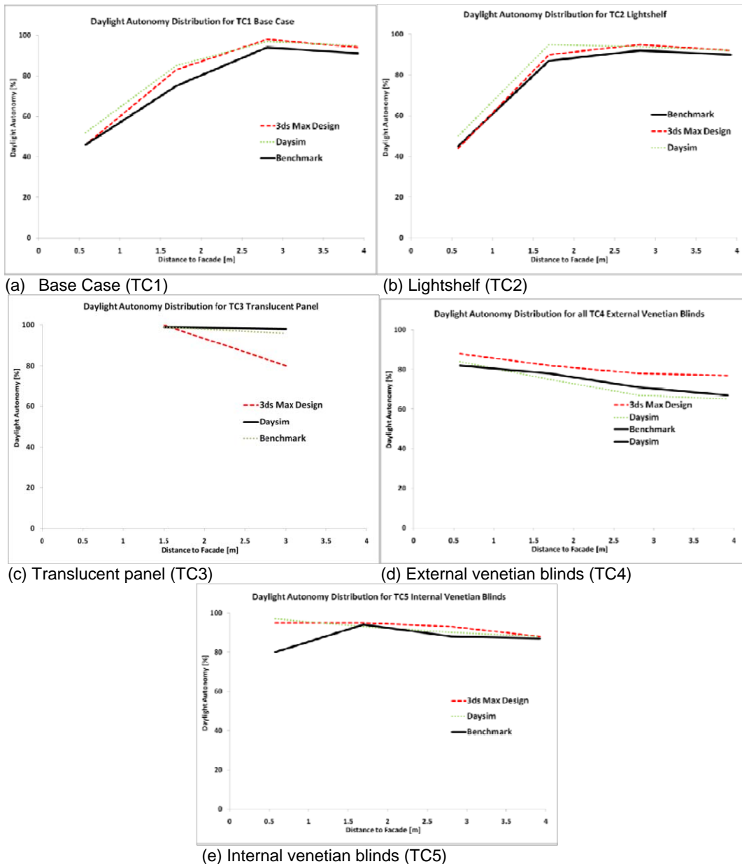
Figure 15: Useful daylight illuminance distributions for the five test cases according to measurements and simulations.
